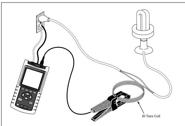
Fig. 1 Example test set up for compact fluorescent lamps
