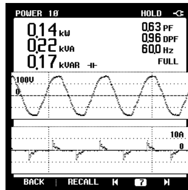
Fig. 2 Compact fluorescent lamp power consumption and current waveform
