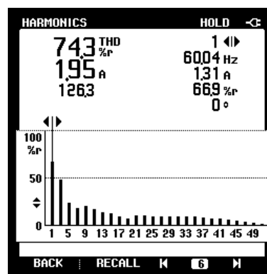
Fig. 3 Compact fluorescent lamp current harmonic spectrum
